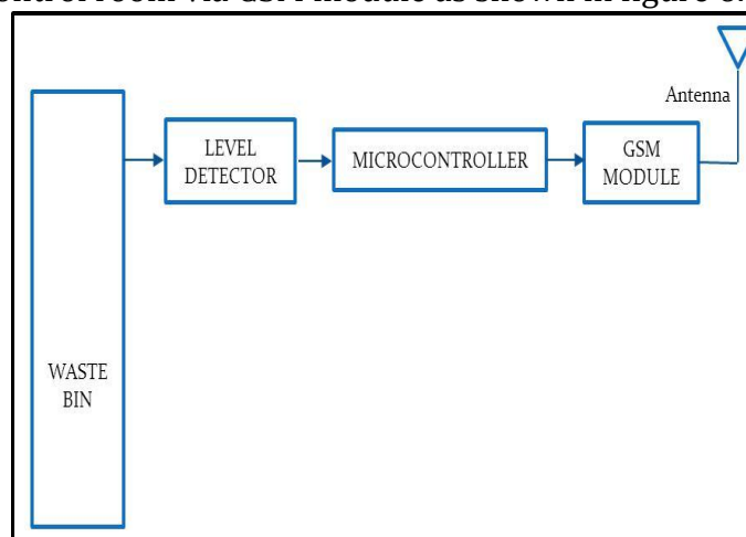
Figure 3: Transmitter Section
