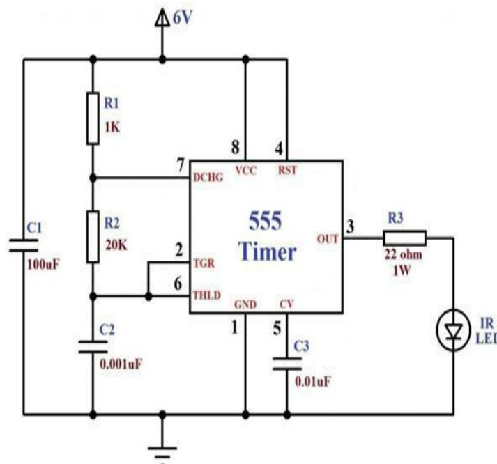
Figure 5: IR Sensor Transmitter
