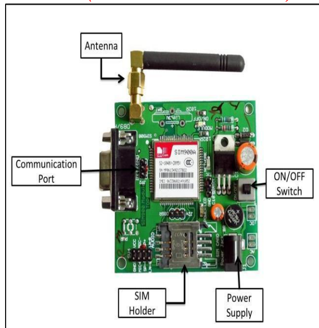
Figure 2: GSM Modem
